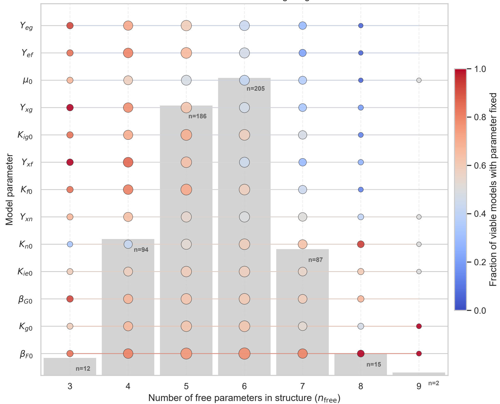
Parameter fixation tree along Stage II
